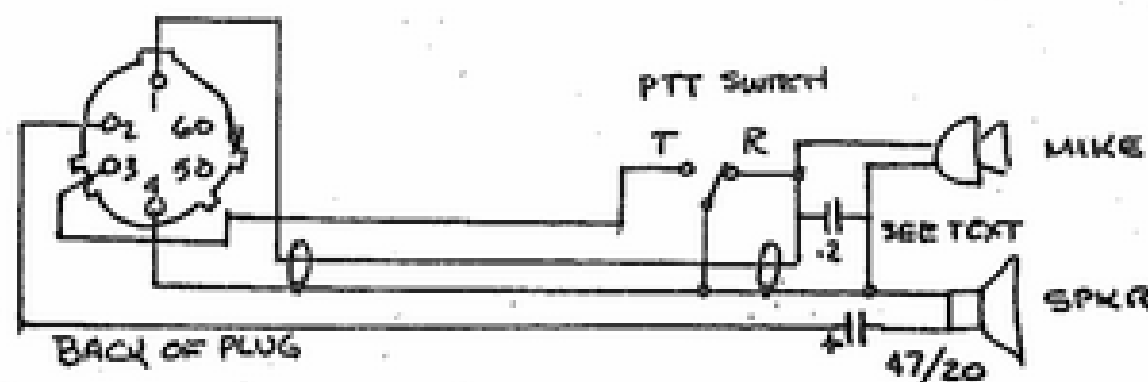
Figure 3. 4 wire cord
