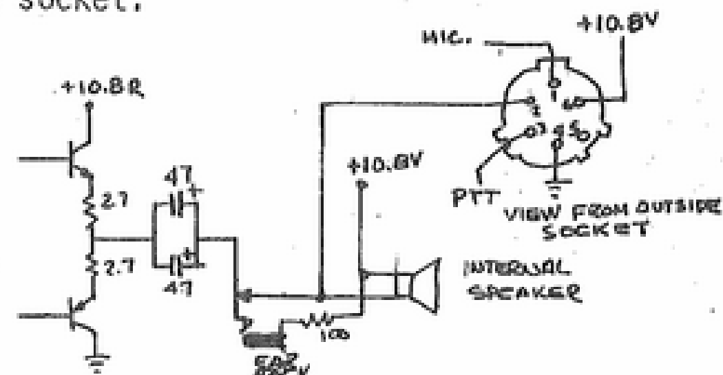
Figure 1 FT-708R Audio
