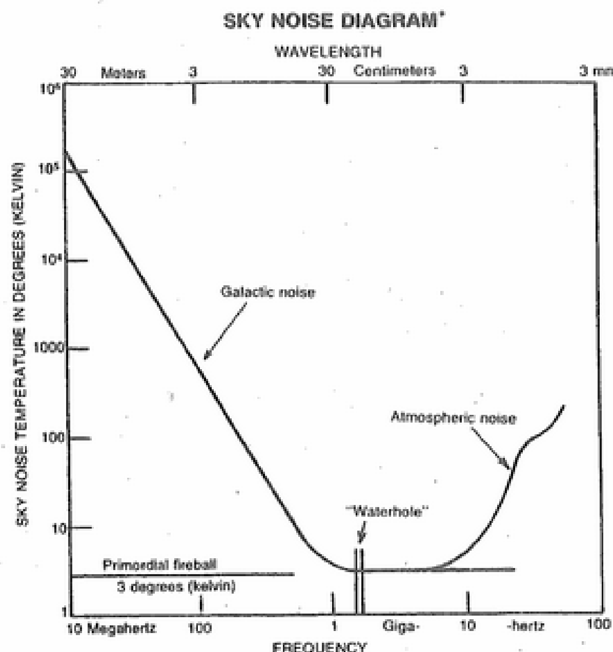
Figure 1. Sky Noise Diagram from J. D. Kraus "Radio Astronomy, McGraw Hill, 1966.
