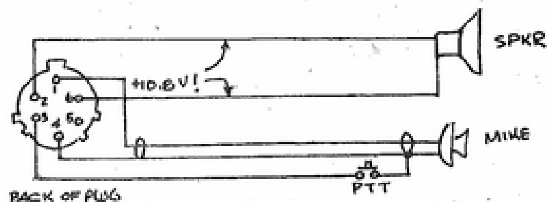
Figure 2. 5 wire cord
