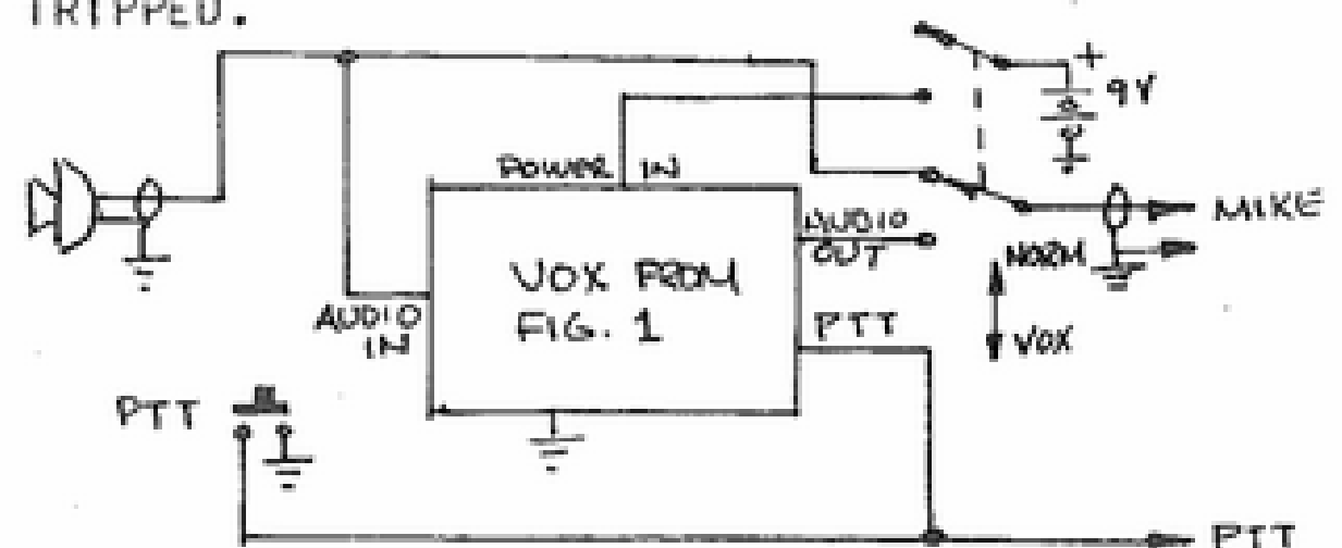
FIGURE 2 VOX INTERFACE
