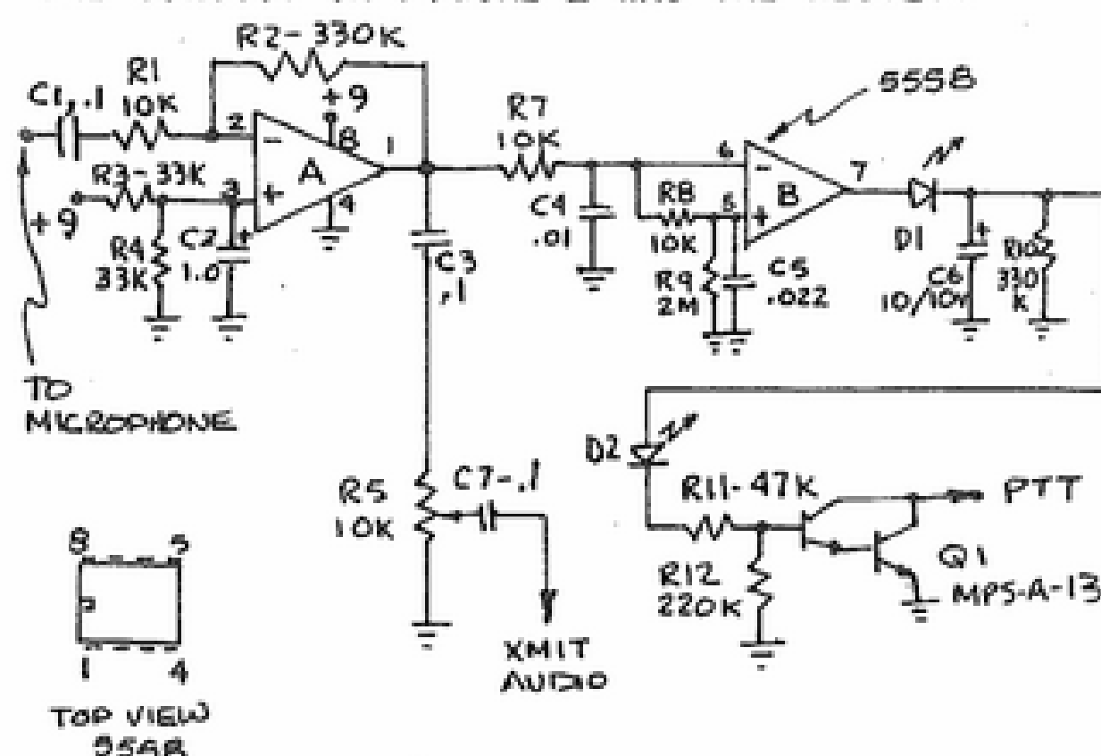
FIGURE 1. VOX FOR HANDHELD
