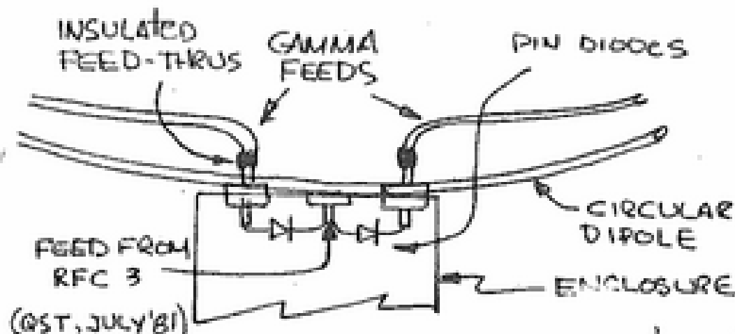
FIGURE 1 PHASE SWITCHER FOR LCD
