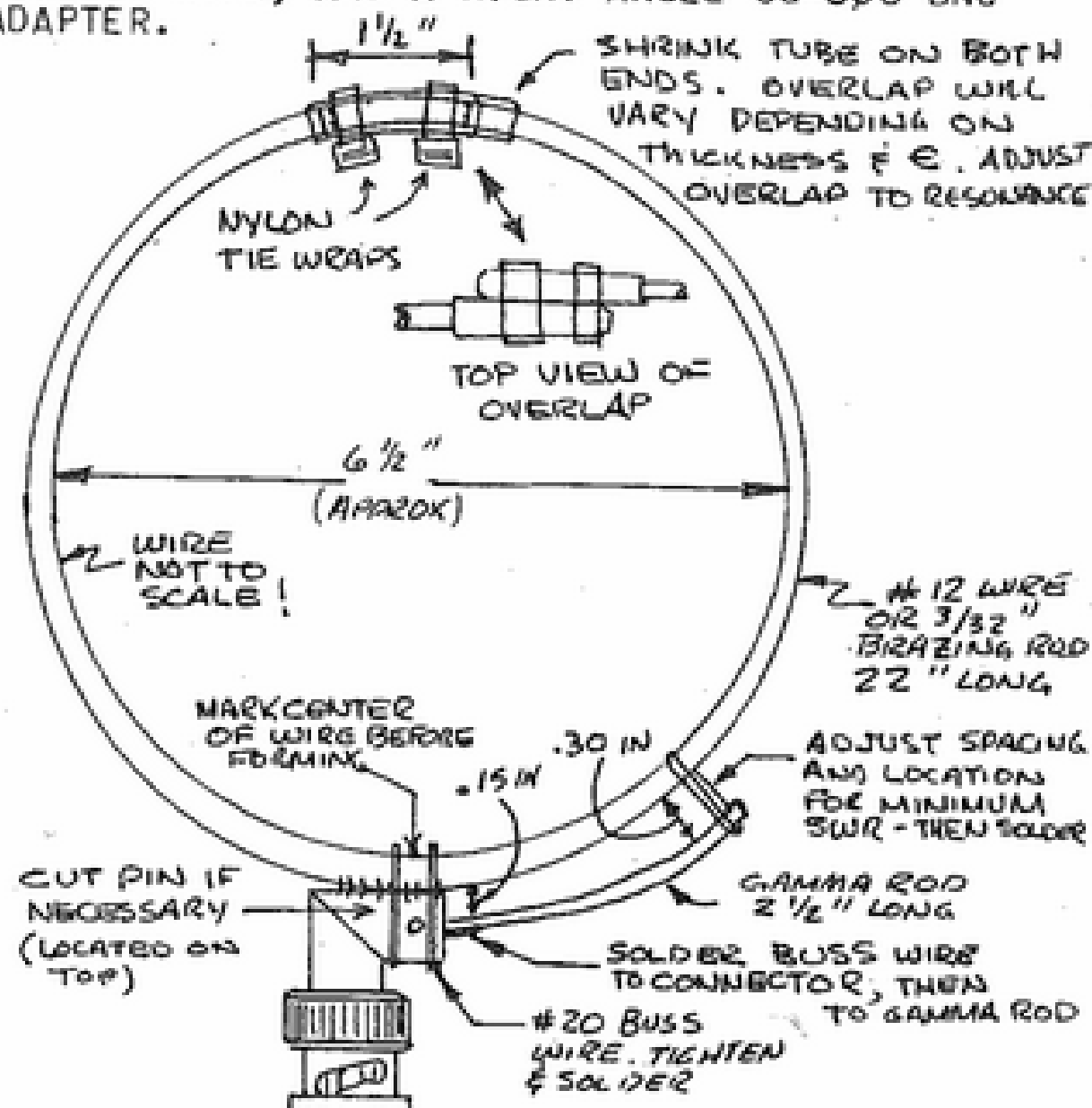
FIGURE 1 LCD - LITTLE CIRCULAR DIPOLE
